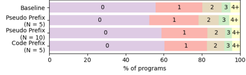
(b) Number of lines in a program where no candidate is correct, i.e. C_l(100) fails.
